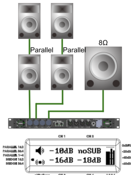
x3 configuration with mix of bridged output on 1st pair of outputs estimated max. output = 1200W + 600Wx2
