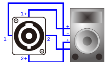
Bi-Amp Connection
