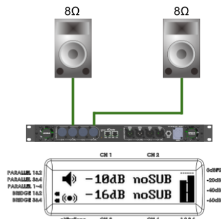
x2 bridge configuration with 8Ω Speakers on each bridged output. estimated max. output = 1200Wx2
