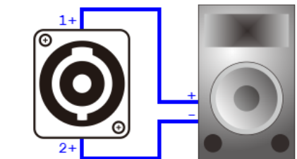
BTL Connection
