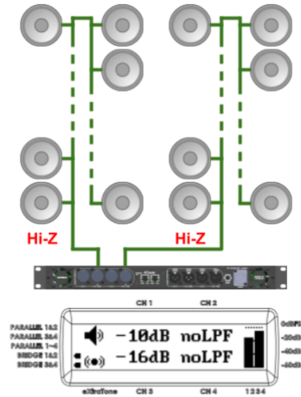
x2 bridge configuration with Parallelized Hi-Z Speakers on each bridged output. estimated max. output = 600Wx2
