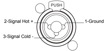
XLR-1/4"TRS Combo socket for direct input
