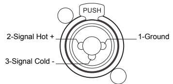
XLR-TRS Combo input
